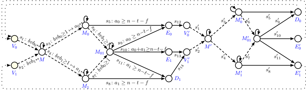
■ Figure 4 The simplified threshold automaton of the Byzantine consensus of Algorithm 1 obtained after model checking the bv-broadcast. Rules s'_j , 1 \leq j \leq 11 , are obtained from s_j by replacing each variable c \in \{a_0, a_1, bvb_0, bvb_1\} with its corresponding one c' .
